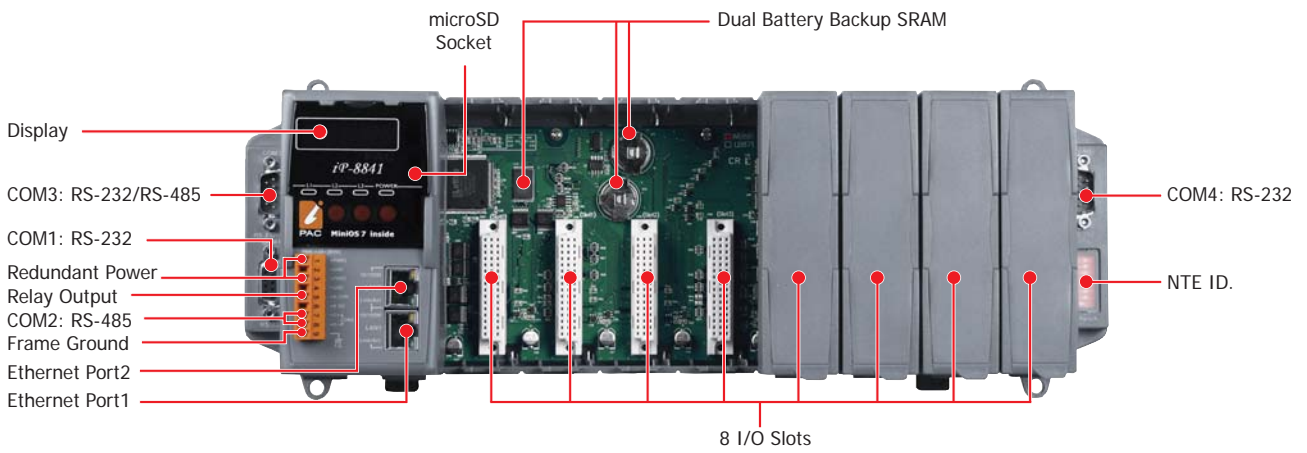
iP-8841/iP-8841-FD
