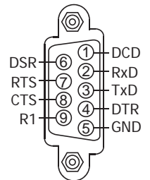
COM4: RS-232
